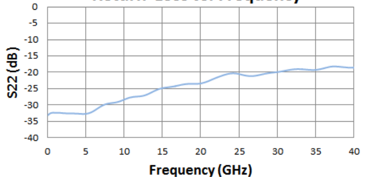
Return Loss vs. Frequency
