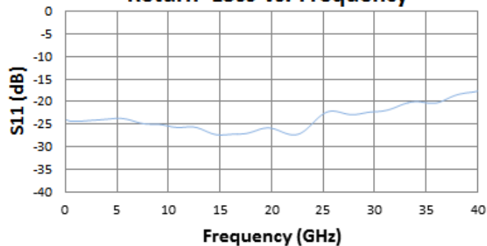
Return Loss vs. Frequency
