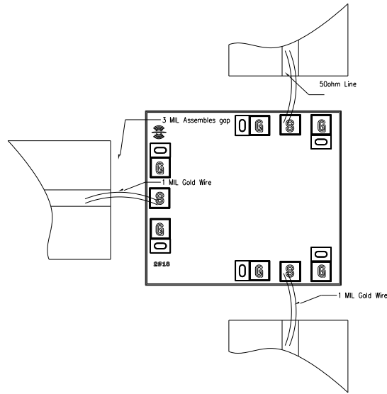
Assembly Diagram
