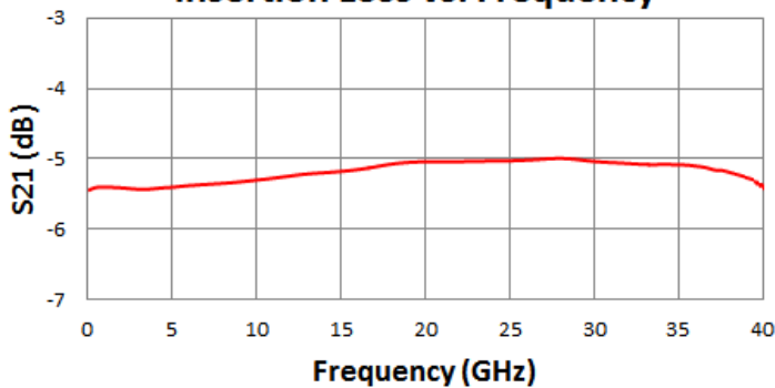
Insertion Loss vs. Frequency
