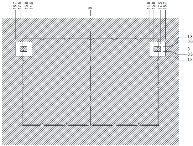
LAND PATTERN
