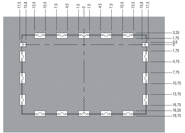
SOLDER RESISTER
