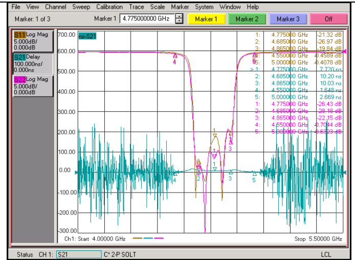
Group Delay
