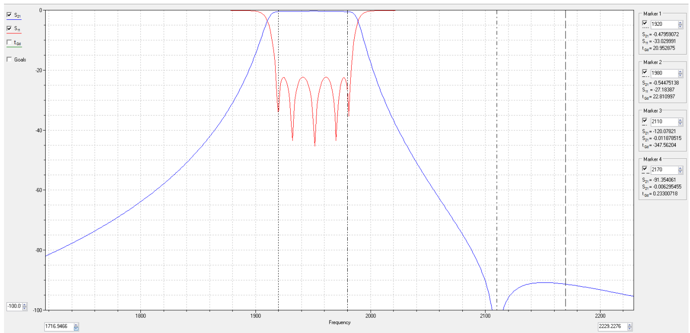
RX path
