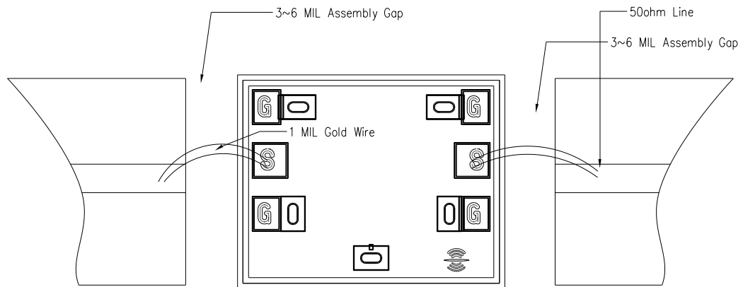
Assembly Diagram
