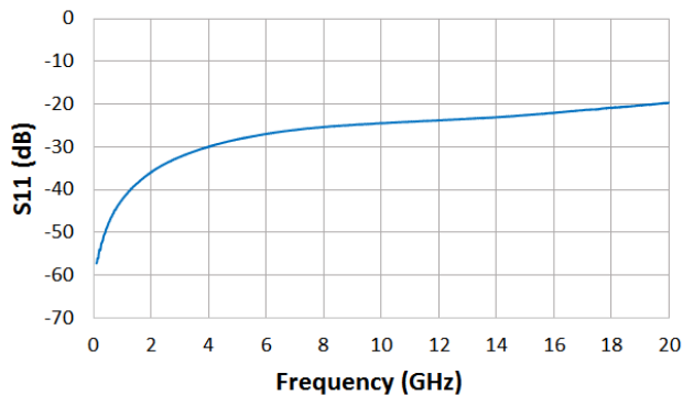
Retrun Loss vs. Frequency
