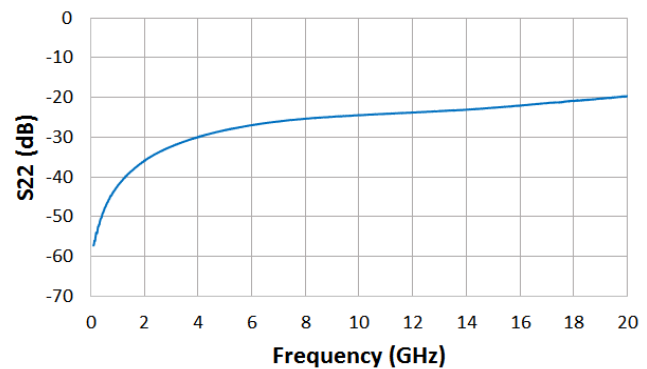
Retrun Loss vs. Frequency
