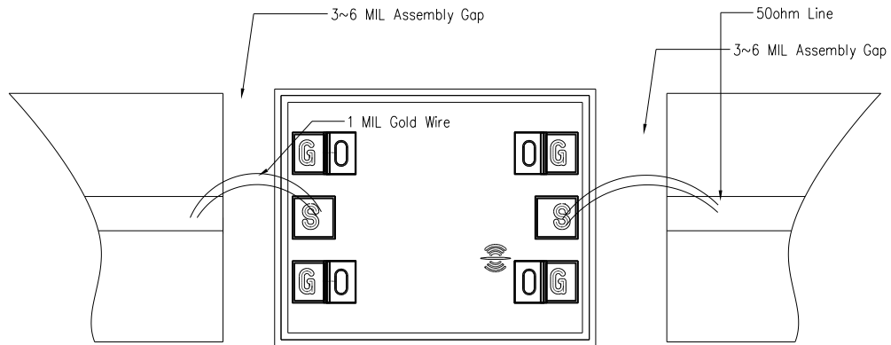
Assembly Diagram
