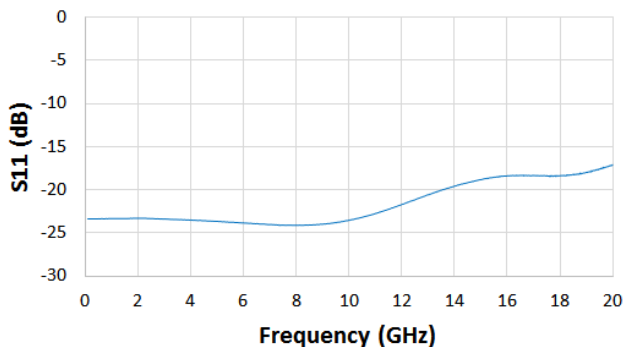
Return Loss vs. Frequency
