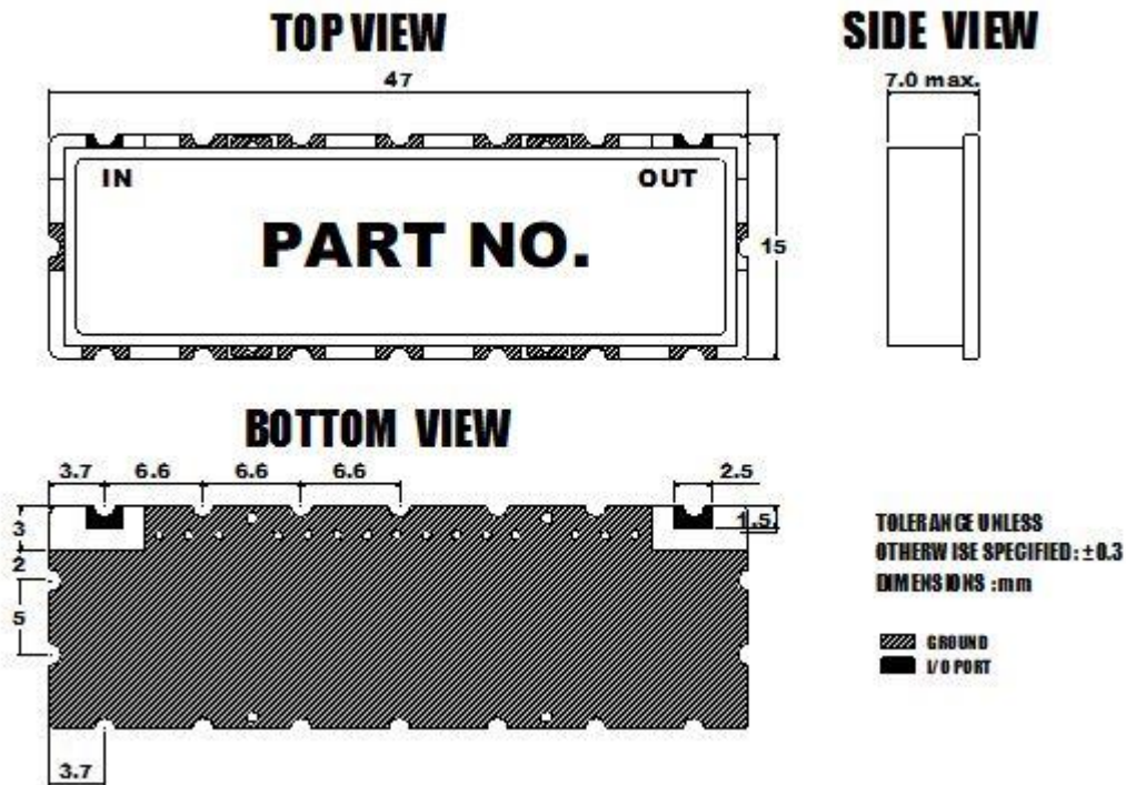
[ Mechanical 2D Drawing ]
