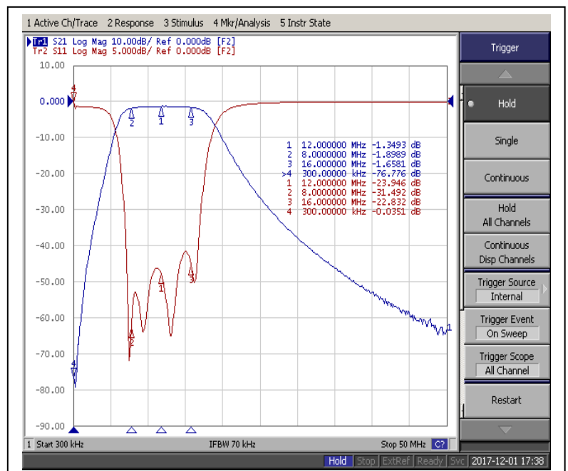
[ TEST CURVE ]
