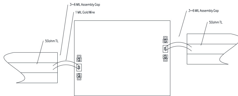
Assembly Diagram
