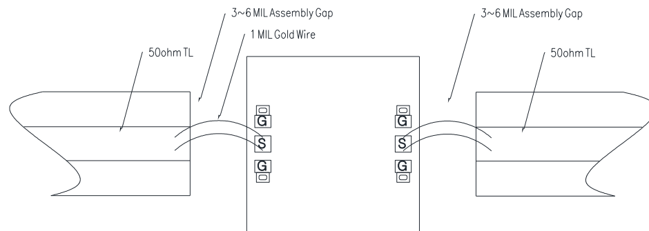
Assembly Diagram
