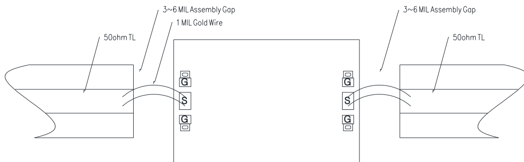
Assembly Diagram
