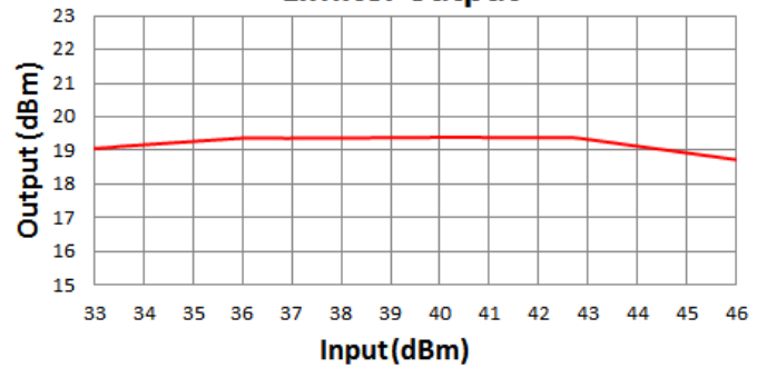
Limiter output
