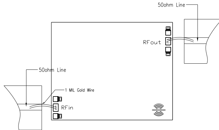
Assembly Diagram
