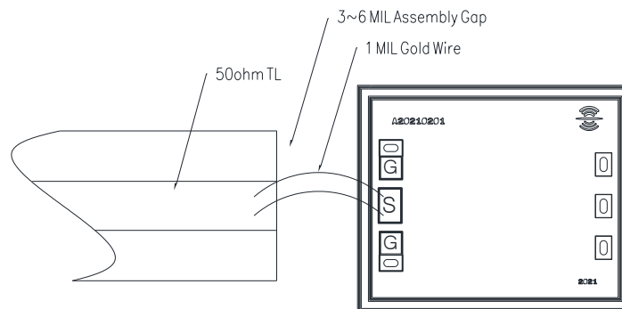
Assembly Diagram
